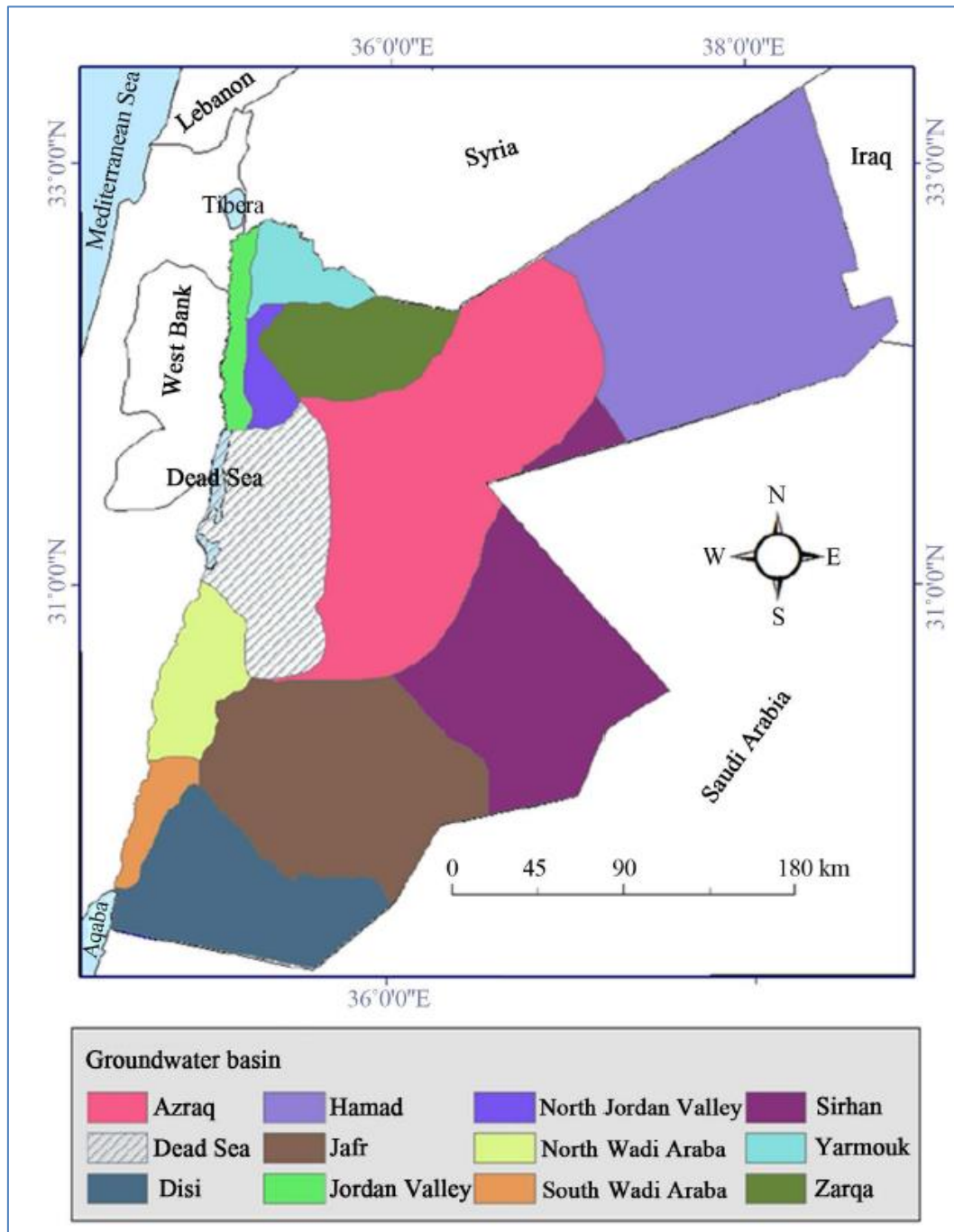
Figure 5-3: Groundwater Basins in Jordan
