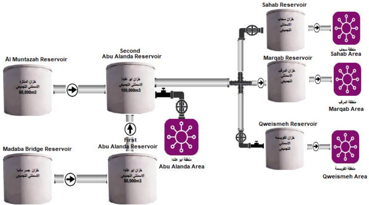
Figure 5-2: Schematic of Water Supply in Sahab – System One
