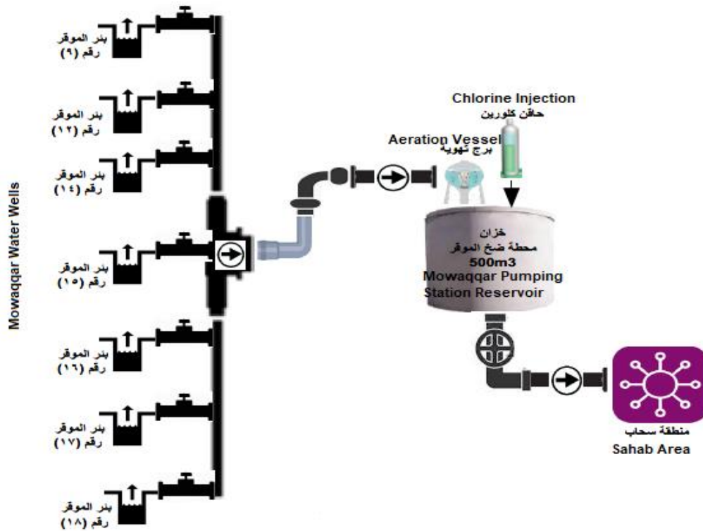
Figure 5-3: Schematic of Water Supply in Sahab – System Two
