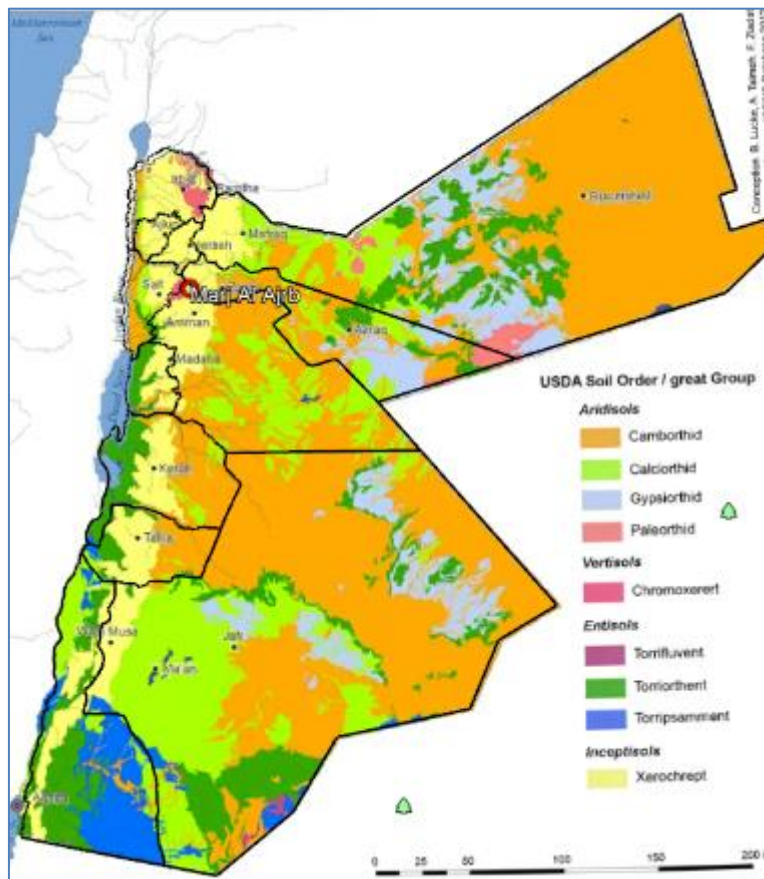
Figure 5-1: Soil Orders and Great Groups in Jordan
