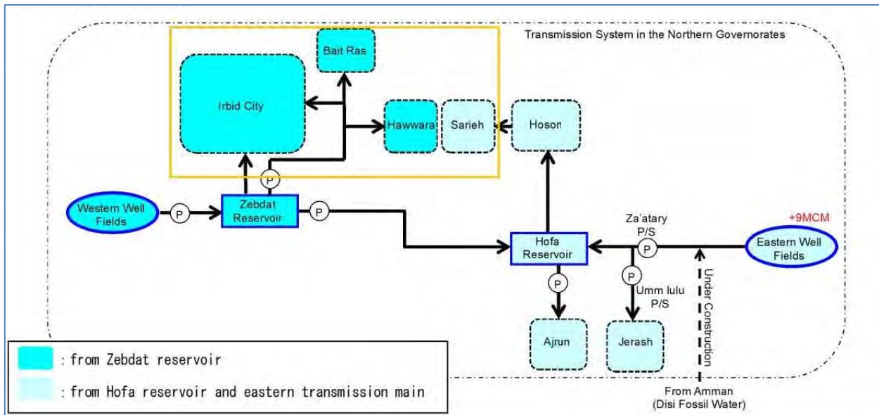
Figure 5-1: Howwara project site water transmission system in Irbid Governorate
